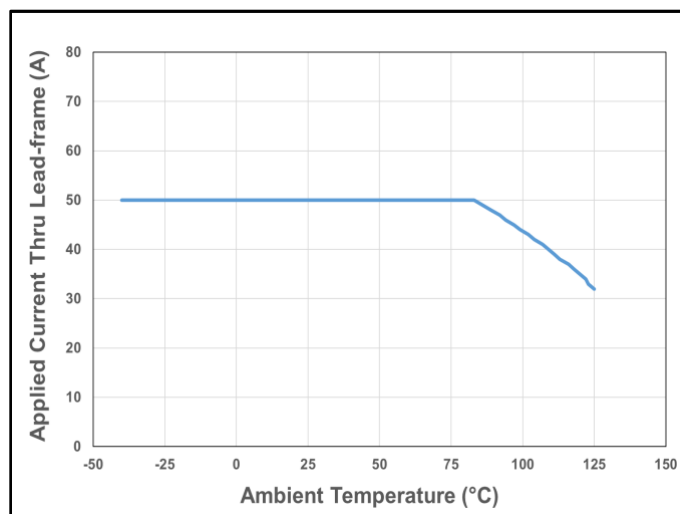
Figure 22. CT433 Current De-rating Curve for 50 A DC
