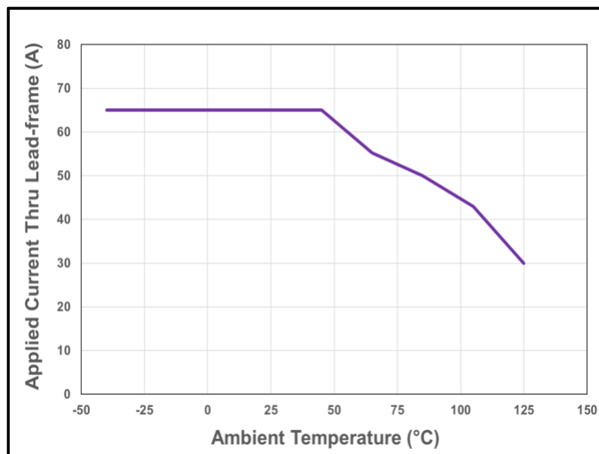
Figure 28. CT433 Current De-rating Curve for 65 A DC
