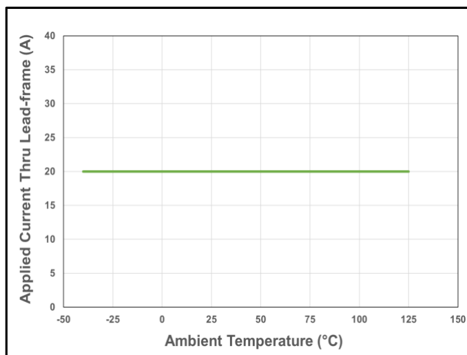
Figure 10. CT433 Current De-rating Curve for 20 A DC
