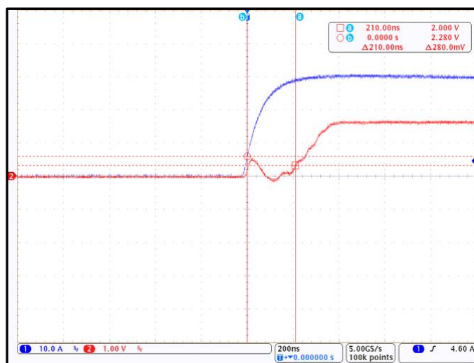
Figure 7. CT433 Propagation Delay; I_P = 30\text{ A}_{PK} and C_L = 100\text{ pF} (Blue = I_{LCC} , Red = V_{OUT} )
