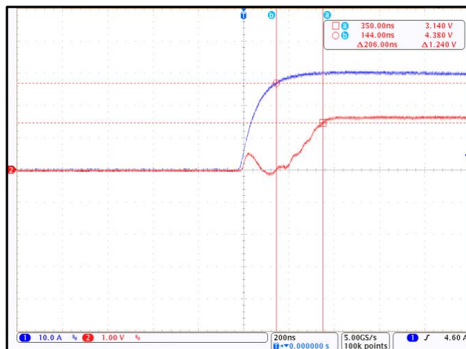
Figure 5. CT433 Response Time; I_P = 30\text{ A}_{PK} and C_L = 100\text{ pF} (Blue = I_{LCC} , Red = V_{OUT} )
