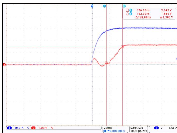
Figure 6. CT433 Rise Time; I_P = 30\text{ A}_{PK} and C_L = 100\text{ pF} (Blue = I_{LCC} , Red = V_{OUT} )
