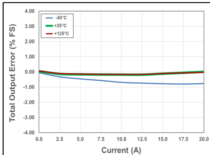
Figure 8. Total Output Error vs. Current vs. Temperature
